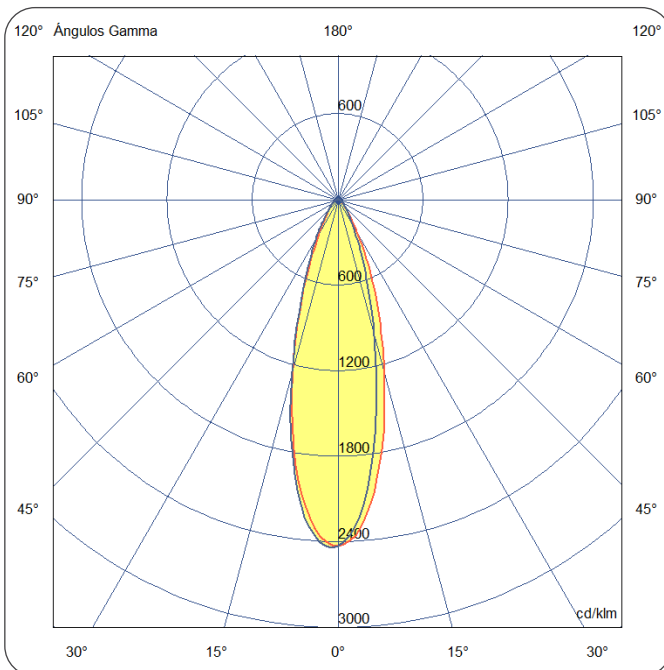
CURVA FOTOMETRICA PHOTOMETRIC CURVE
