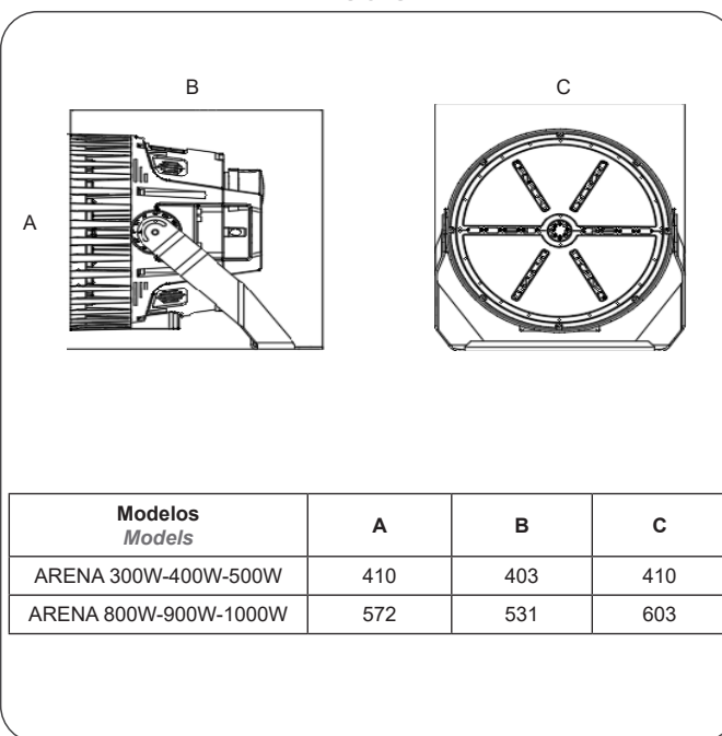
DIMENSIONES DIMENSIONS
